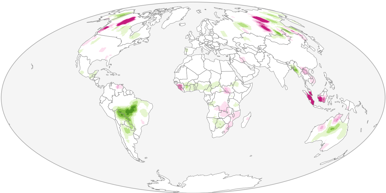
Difference from average emissions (grams of carbon per meter 2 per year)
